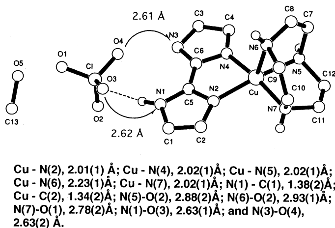
Fig. 3. ORTEP view of the complex [Cu II (tacn)(Hbim)](ClO 4 )·MeOH ( 3 ).
